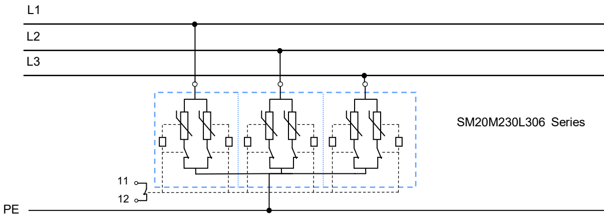
FIGURE 1 Three-phase circuit protection (20 kA)
